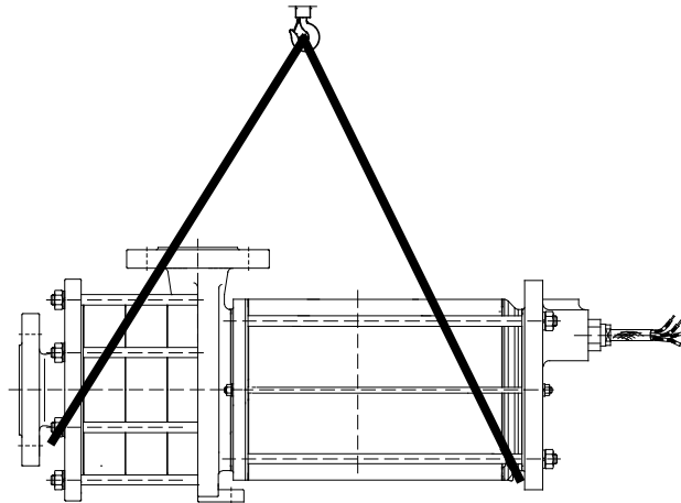
Abb. 5: Hebezeug befestigen an Pumpenaggregat
